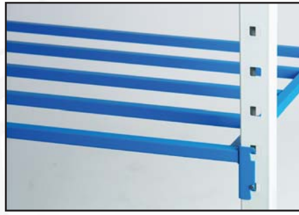
Standard tubular shelf. U.D.L. capacity 250kg. Supplied with retaining pins.
