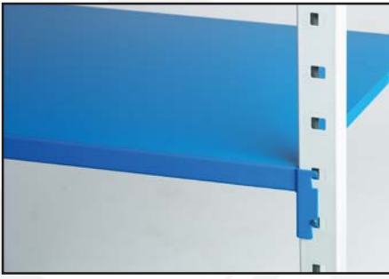
Metal shelf. U.D.L. capacity 250kg. Supplied with retaining pins.
